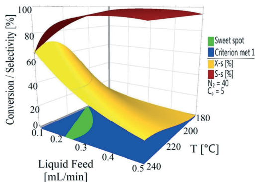
Fig. 8 Sweet spot plot based on objectives of >40% conversion and >99% selectivity in single-pass mode for varying temperature ( 180\text{--}240 \text{ }^\circ\text{C} ) and liquid feed flow ( 0.1\text{--}0.5 \text{ mL min}^{-1} , 0.7\text{--}3.3 \text{ m}^3 \text{ m}^{-2} \text{ h}^{-1} at STP) at fixed nitrogen flow ( 40 \text{ mL min}^{-1} , 266.4 \text{ m}^3 \text{ m}^{-2} \text{ h}^{-1} at STP) and substrate concentration ( 5 \text{ wt}\% ).
