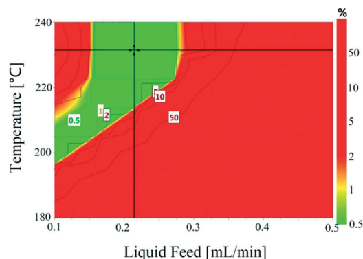
Fig. 9 Design space for the conversion of 1,4-cyclohexanedione in single-pass mode as a function of temperature ( 180\text{--}240 \text{ }^\circ\text{C} ) and liquid feed flow ( 0.1\text{--}0.5 \text{ mL min}^{-1} , 0.7\text{--}3.3 \text{ m}^3 \text{ m}^{-2} \text{ h}^{-1} at STP). The green area is the operating window to meet the desired specification, with the red area indicating risk of failure.
