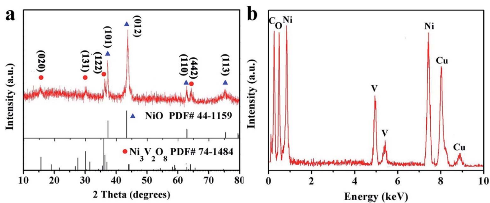
Fig. 2 (a) XRD and (b) EDS pattern of NiO/ \text{Ni}_3\text{V}_2\text{O}_8 NPs.
