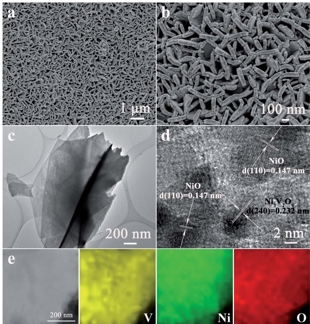
Fig. 3 (a and b) SEM and (c) TEM images of NiO/ \text{Ni}_3\text{V}_2\text{O}_8 NPs. (d) High resolution TEM image of NiO/ \text{Ni}_3\text{V}_2\text{O}_8 NPs. (e) The scan TEM image and the corresponding EDS elemental mapping images of Ni, V, and O.
