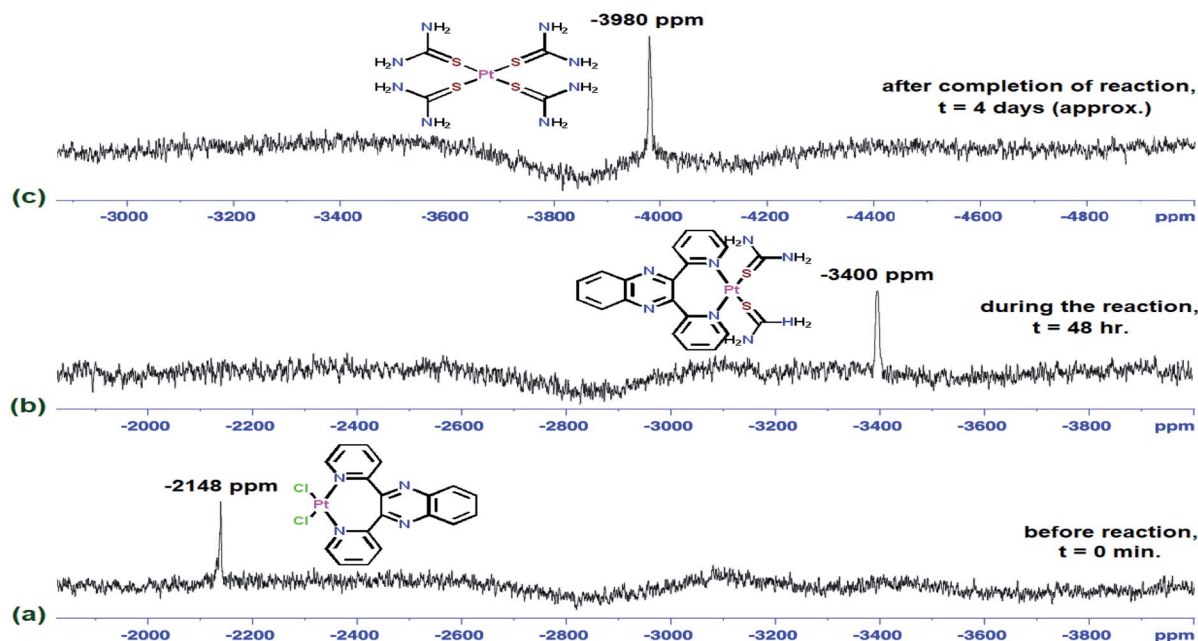
Fig. 6 Time-dependent ^{195}\text{Pt} -NMR chemical shifts of \text{bmqPtCl}_2 in DMSO medium with excess TU; reaction was monitored before (a), at 48 h (b) and after completion (c).
