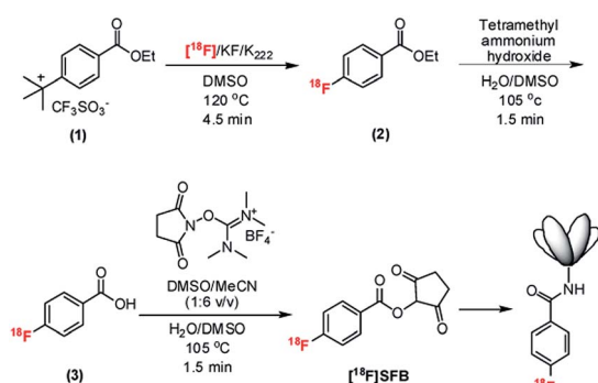
Fig. 1 Overall radiosynthetic scheme of [ ^{18}\text{F} ]SFB on the EWOD chip and the conjugation of the ^{18}\text{F} -labeled prosthetic group to the PSCA-diabody. The conjugation is performed in sodium-borate buffer (SBB, 50 \mu\text{mol L}^{-1} , pH 8.7) and incubated for 10 min at 34 ^\circ\text{C} . Cartoon of diabody is not to scale.
