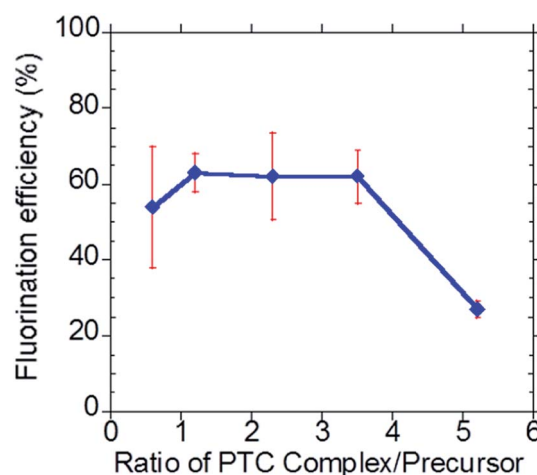
Fig. 3 Investigation of the effect of the phase transfer catalyst complex ( \text{K}^+/\text{K}_{2.2.2} ) to precursor ratio.
