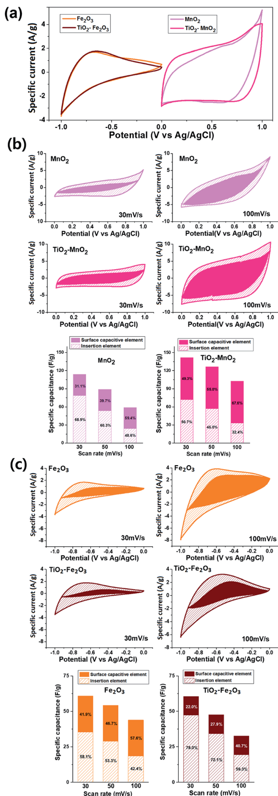
Fig. 2 Cyclic voltammograms of the \text{Fe}_2\text{O}_3 , \text{TiO}_2 - \text{Fe}_2\text{O}_3 , \text{MnO}_2 , \text{TiO}_2 - \text{MnO}_2 electrodes at a scan rate of 30 \text{mV s}^{-1} (a) and deconvolutions of the total capacitance into surface element (solid part) and insertion element (shaded part) for the (b) \text{TiO}_2 - \text{MnO}_2 and (c) \text{TiO}_2 - \text{Fe}_2\text{O}_3 electrodes measured at 30 and 100 \text{mV s}^{-1} . The bar graphs represent the contribution of each element at various scan rates.
