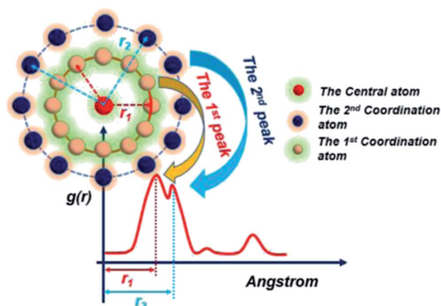
Fig. 2 RDF schematic.
