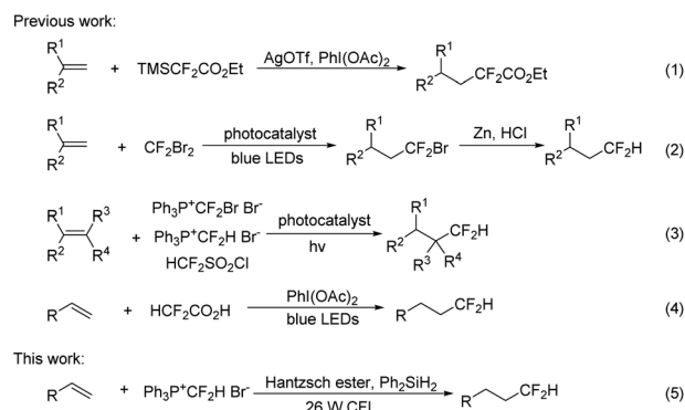
Scheme 1 Hydrodifluoromethylation of alkenes.
