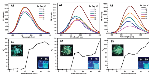
Fig. 3 Fluorescent spectra of TPE-L-Glu, cis -TPE-L-DGlu and trans -TPE-L-DGlu in THF/water mixed solvents with different f_w (A1-A3); plot of I_0/I values versus f_w (B1-B3), where I_0 represents the emission intensity in THF. Concentration: 1 \times 10^{-5} M; excitation wavelength: 340 nm. Inset: Photographs of TPE-L-Glu, cis -TPE-L-DGlu and trans -TPE-L-DGlu in solid and THF/water mixtures with 0 and 99% f_w under 365 nm UV lamp.
