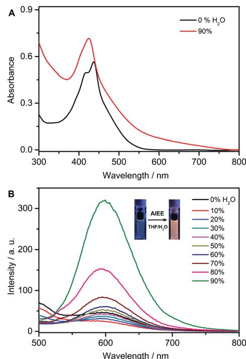
Fig. 4 AIEE behavior of the copolymer. (A) Absorption and (B) emission spectra of copolymer P(NIPAM-co-EM) (15.6 \mu M) in H 2 O/THF mixtures with different f_w . \lambda_{ex} = 430 nm; inset (B): fluorescence images of the P(NIPAM-co-EM) ( f_w = 0 and 90%) under UV light irradiation.
