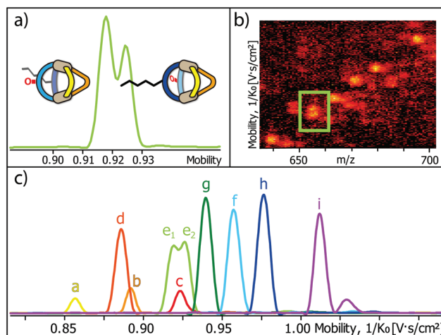
Fig. 5 (a) High resolution TIMS mobilogram allowing the discrimination of cis - [\text{Pd}_2\text{L}^{\text{C}}\text{L}^{\text{F}}\text{L}^{\text{P}}\text{L}^{\text{P}'}]^{4+} and trans - [\text{Pd}_2\text{L}^{\text{C}}\text{L}^{\text{F}}\text{L}^{\text{P}}\text{L}^{\text{P}'}]^{4+} ; (b) partial heat map and (c) full mobilogram of the simultaneous ion mobility measurement of all ten coordination cages; assignments a–i correspond to cages shown in Fig. 6.
