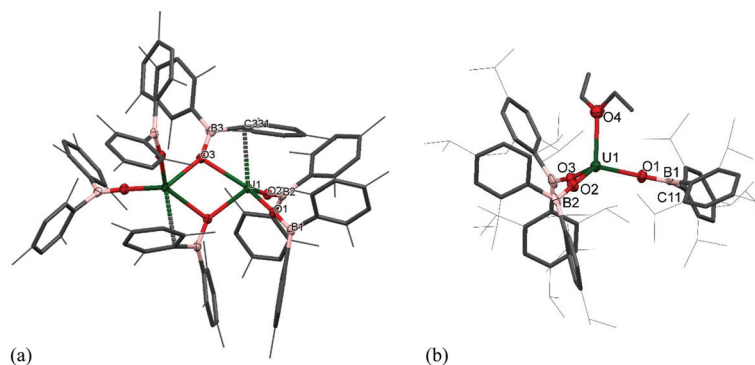
Fig. 1 Displacement ellipsoid drawing of the molecular structure of (a) \mathbf{1}^m and (b) \mathbf{1}^t\text{-Et}_2\text{O} . The hydrogen atoms are omitted and the mesityl and triisopropylphenyl groups are depicted as wireframe and capped sticks for clarity. The thermal ellipsoids are displayed at 50% probability.
