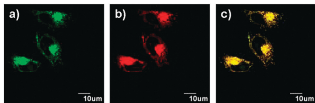
Fig. 18 Probe 13 co-localizes to lysosomes in live MCF-7. Cells were stained with: (a) 1 \mu\text{M} LysoTracker Green, (b) 10 \mu\text{M} Probe 13 . (c) Areas of co-localization appear in yellow. Probe 13 and LysoTracker Green were excited at 559 nm and 488 nm, respectively. The fluorescence images were recorded at 575–620 nm (Probe 13 ) and 495–515 nm (LysoTracker Green), respectively. Copyright 2012 Royal Society of Chemistry.
