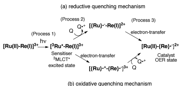
Scheme 1 Reductive and oxidative pathways in the photochemical formation of the OERS of \text{RuRe(X)} .
