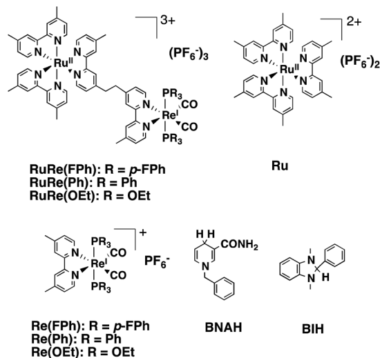
Chart 1 Structures and abbreviations of the \text{Ru(II)}\text{--Re(I)} binuclear complexes, the model complexes of their subunits ( \text{Ru} and \text{Re(X)} ), \text{BNAH} , and \text{BIH} .
