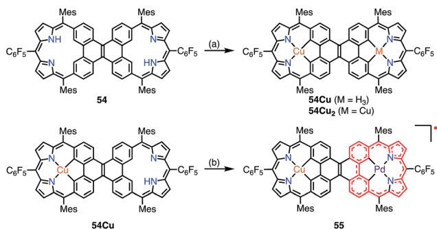
Fig. 17 Metalation of dicarbacorroles with Cu(III) and Pd(II). (a) \text{Cu}(\text{OAc})_2 \cdot \text{H}_2\text{O} in \text{CHCl}_3 , reflux, 48 h; (b) \text{Pd}(\text{PhCN})_2\text{Cl}_2 in PhCN, 180^\circ\text{C} , 2 h, 89%.
