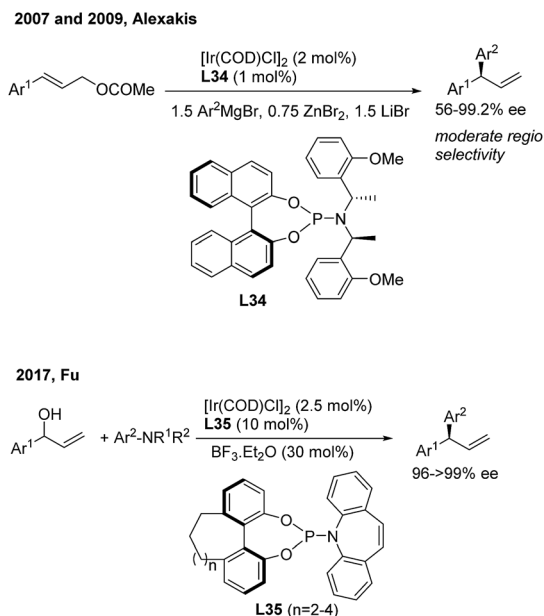
Scheme 23 Ir(i)-catalyzed AAAr using chiral phosphoramidite ligands.
