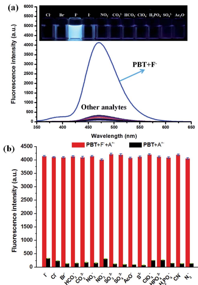
Fig. 6 (a) Fluorescence spectra of PBT in the presence of various anions. [PBT] = 10\ \mu\text{M} , [A^-] = 20\ \mu\text{M} , in a mixture of THF and Tris buffer solution (pH 8.0), (1 : 9, v/v), \lambda_{\text{ex}} = 335\ \text{nm} , \lambda_{\text{em}} = 470\ \text{nm} . Inset: direct observation of fluorescence emission difference of the probe PBT ( 10\ \mu\text{M} ) under UV irradiation (365 nm) in the presence of different anions. Left to right: \text{Cl}^- , \text{Br}^- , \text{I}^- , \text{F}^- , \text{NO}_2^- , \text{CO}_3^{2-} , \text{HCO}_3^- , \text{ClO}_4^- , \text{H}_2\text{PO}_4^- , \text{SO}_4^{2-} and \text{AcO}^- . (b) The selectivity of PBT in the presence of various anions.
