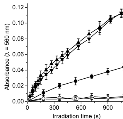
Fig. 3 Time course of NBT reduction as an increase in the absorption at \lambda = 560 nm in DMF/10% water. Samples contain NBT (0.2 mM), NADH (0.5 mM) and \text{TCP}-\text{C}_{60} ( \blacktriangle ) (1.2 \mu\text{M} ) or \text{TCP}-\text{C}_{60}^{4+} ( \blacktriangledown ) (1.2 \mu\text{M} ) in DMF/10% water irradiated with light at \lambda_{\text{irr}} = 428 nm. Controls: NBT and NADH ( \bullet ), \text{TCP}-\text{C}_{60} and NBT ( \Delta ); \text{TCP}-\text{C}_{60}^{4+} and NBT ( \nabla ).
