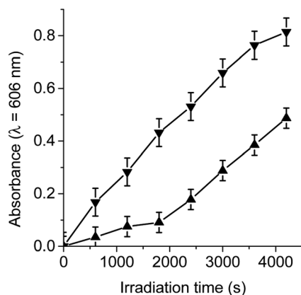
Fig. 2 Time course of \text{MV}^{2+} (0.8 mM) reduction as an increase in the absorption at \lambda = 606 nm sensitized by \text{TCP}-\text{C}_{60} ( \blacktriangle ) (3.0 \mu\text{M} ) and \text{TCP}-\text{C}_{60}^{4+} ( \blacktriangledown ) (3.0 \mu\text{M} ) containing TMN (0.4 mM) after 10 min irradiation periods with light at \lambda_{\text{irr}} = 433 nm under an argon atmosphere in DMF/5% water.
