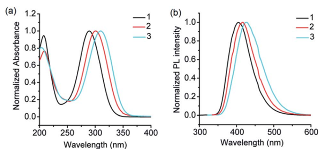
Fig. 5 (a) UV-visible absorption spectra of 1 , 2 and 3 ( \lambda_{\text{max}} for the n \rightarrow \pi^* transition = 289, 300 and 309 nm), and (b) photoluminescence spectra of 1 , 2 and 3 ( \lambda_{\text{em}} = 405, 415 and 425 nm) in acetonitrile (see Scheme 1 for the structures of 1–3 ).
