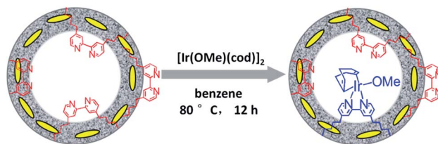
Scheme 3 Synthetic route for the molecular heterogeneous solid catalyst Ir(cod)-BP 0.3 -NT.
