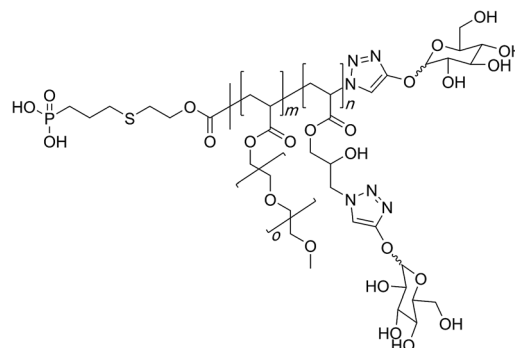
Fig. 2 Chemical structure of the glycopolymers synthesised through use of azide-epoxy reaction on the PGMA scaffold.
