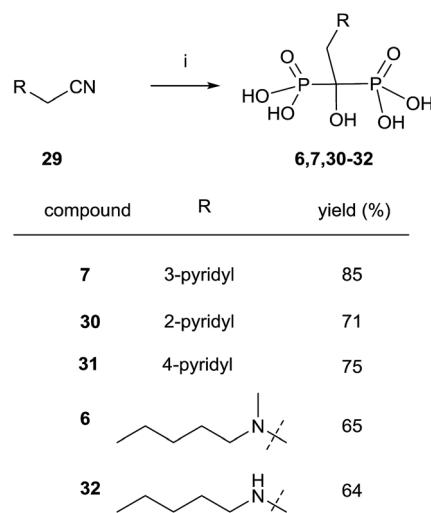
Scheme 9 Reagents and conditions: (i) \text{CH}_3\text{SO}_3\text{H} , 8 h, 100 °C; then \text{PCl}_3 , 70 °C, 5 h; then \text{H}_2\text{O} , 15 h, 98 °C.
