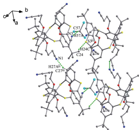
Fig. 50 Partial packing structure of 54 , showing intermolecular H-bonds.
