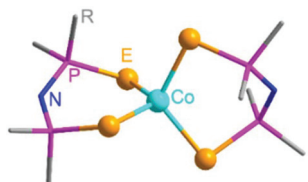
Fig. 1 Molecular structure diagram of Co([EPR 2 ) 2 N] 2 (E = S, Se, Te; R = Ph, i Pr). The hydrogen atoms and the R groups are not shown for clarity.
