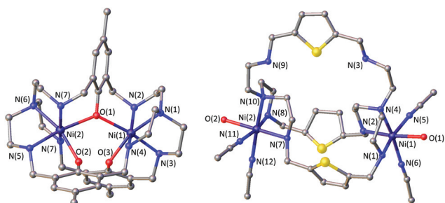
Fig. 1 Molecular structures of [\text{Ni}_2\text{L}_\text{A}^{\text{OH,Me}}](\text{ClO}_4)_2 (left) and [\text{Ni}_2\text{L}_\text{A}^{\text{Thio}}](\text{ClO}_4)_4 (right). Hydrogen atoms and counter ions were omitted for clarity.
