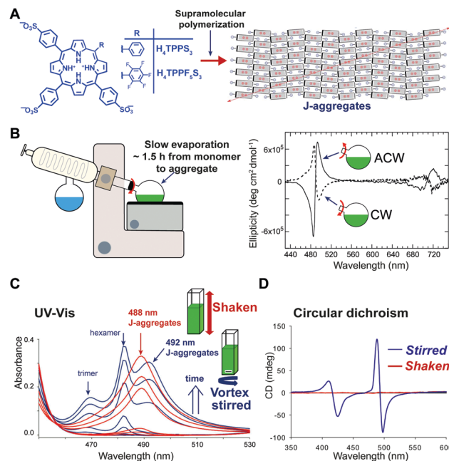
Fig. 10 Pathway selection via hydrodynamic fields. (A) Diprotated 4-sulfonatophenyl meso -substituted porphyrins self-assemble hierarchically to give J-aggregates. This aggregates are based on an intrinsically chiral 2D sheet structure, that depending on the porphyrin meso -substitution pattern, and on the preparation protocol can assemble further to give bi- or multi-layered structures (cf. ref. 41 and 44). Adapted from ref. 44 with permission from The Royal Society of Chemistry. (B) Chiral sign selection in H_4TPPS_3 J-aggregation depending on the direction of stirring during the rotary evaporation of diluted monomeric solutions to assembled ones. Adapted from ref. 42 with permission from The American Association for the Advancement of Science, copyright 2001. (C) Typical evolution of the aggregation of H_4TPPF_5S_3 under shaking (uniform mixing) or magnetic stirring (imperfect mixing) conditions, as monitored by UV-Vis spectroscopy. Adapted from ref. 45 with permission from The Royal Society of Chemistry. (D) CD spectra of H_4TPPF_5S_3 aggregates obtained under vigorous-shaking and magnetic stirring. Adapted from ref. 46 with permission from Wiley-VCH Verlag GmbH & Co., copyright 2012.
