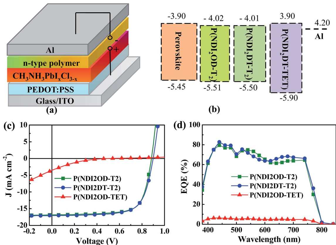
Fig. 1 (a) Device structure of HPSCs described in this study. (b) Energy levels of the perovskite and of the three n-type polymers. (c) J-V curves under illumination and (d) EQE of the devices using the three different n-type polymers as EELs.
