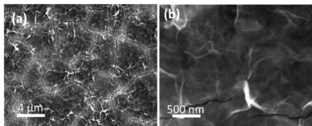
Fig. 2 (a and b) SEM images of \text{Co}(\text{OH})_2 electrodeposited on to a Au electrode at a potential of -0.95 V for 60 s in a solution of 10\text{ mM Co}(\text{NO}_3)_2 \cdot 6\text{H}_2\text{O} .
