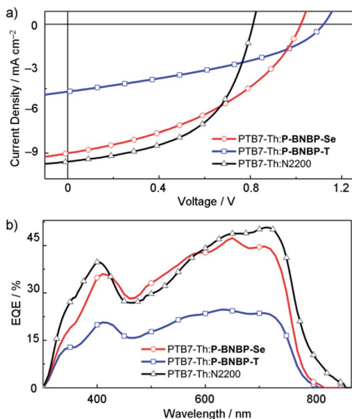
Fig. 4 (a) J - V curves and (b) EQE spectra of the all-PSC devices based on the PTB7-Th:P-BNBP-Se, PTB7-Th:P-BNBP-T and PTB7-Th:N2200 blends, respectively.
