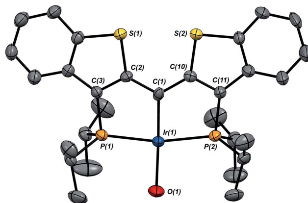
Fig. 3 Molecular structure of 3 \cdot \text{OH} . Hydrogen atoms have been omitted for clarity. Displacement ellipsoids are shown at the 50% probability level. Selected bond lengths (Å): \text{Ir}(1)-\text{P}(1) , 2.2904(13); \text{Ir}(1)-\text{P}(2) , 2.2817(13); \text{Ir}(1)-\text{C}(1) , 1.943(5); \text{Ir}(1)-\text{O}(1) , 2.004(4). Selected bond angles ( ^\circ ): \text{C}(1)-\text{Ir}(1)-\text{O}(1) , 175.5(2); \text{P}(1)-\text{Ir}(1)-\text{P}(2) , 166.08(5).
