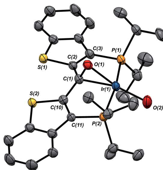
Fig. 4 Molecular structure of 1 \cdot \text{OH} . Hydrogen atoms have been omitted for clarity. Displacement ellipsoids are shown at the 50% probability level. Selected bond lengths (Å): \text{Ir}(1)-\text{P}(1) , 2.3110(10); \text{Ir}(1)-\text{P}(2) , 2.3135(10); \text{Ir}(1)-\text{C}(1) , 2.078(4); \text{Ir}(1)-\text{O}(1) , 2.084(3); \text{Ir}(1)-\text{O}(2) , 1.972(4); \text{C}(1)-\text{O}(1) , 1.359(5). Selected bond angles ( ^\circ ): \text{C}(1)-\text{Ir}(1)-\text{O}(1) , 38.12(13); \text{C}(1)-\text{O}(1)-\text{Ir}(1) , 70.7(2); \text{Ir}(1)-\text{C}(1)-\text{O}(1) , 71.2(2); \text{P}(1)-\text{Ir}(1)-\text{P}(2) , 166.23(4).
