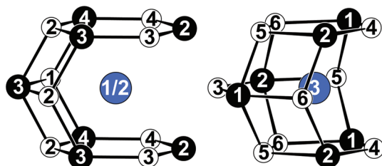
Fig. 4 Coordination environments surrounding the Ce1/2 (left) and Ce3 (right) atoms in the crystal structure of Ce_3Pt_4Ge_6 . Ce atoms are depicted as blue, Pt atoms as black and Ge atoms as open white circles.
