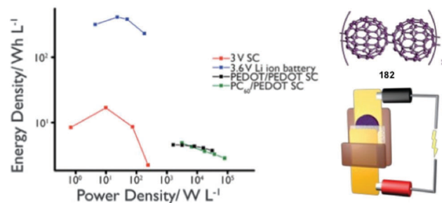
Fig. 28 Ragone plot of symmetric PEDOT SC and asymmetric 182 SC plotted with commercially available 3 V 0.2 F activated carbon SC and a 3.6 V 110 mA h lithium-ion battery. Adapted from ref. 174.
