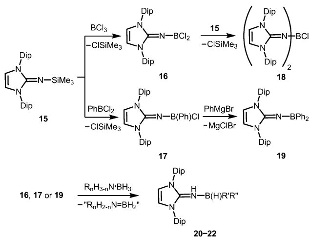
Scheme 6 Conversion of the imino trimethylsilane 15 to the imino boron chloroboranes 16–18 and the imino diphenylborane 19 . Formation of the imine–borane adducts via abstraction of dihydrogen from amine–borane adducts.
