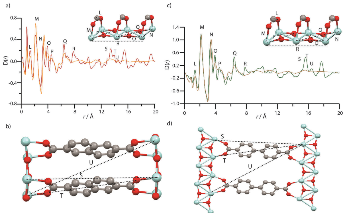
Fig. 7 (a) PDF data for MIL-140B and a MIL-140B * . Labels of peaks below 8 Å correspond to the indicated correlations in the ZrO inorganic chains (inset). (b) Two ZrO chains linked by 2,6- ndc , and the distances corresponding to the longer r features in (a). (c) PDF data for MIL-140C and a MIL-140C . Labels of peaks below 8 Å correspond to the indicated correlations in the ZrO inorganic chains, as in MIL-140B (inset). (d) Two ZrO chains linked by bpdc , and the distances corresponding to the longer r features in (a). Zr – light blue, O – red, C – gray, H – omitted. To facilitate assignment of features, partial PDFs were calculated using the PDFgui software (Fig. S7–S9, ESI†). 57 All PDFs of crystalline species are, as expected, dominated by correlations involving Zr, due to the larger X-ray scattering cross section of Zr relative to C, O and H.
