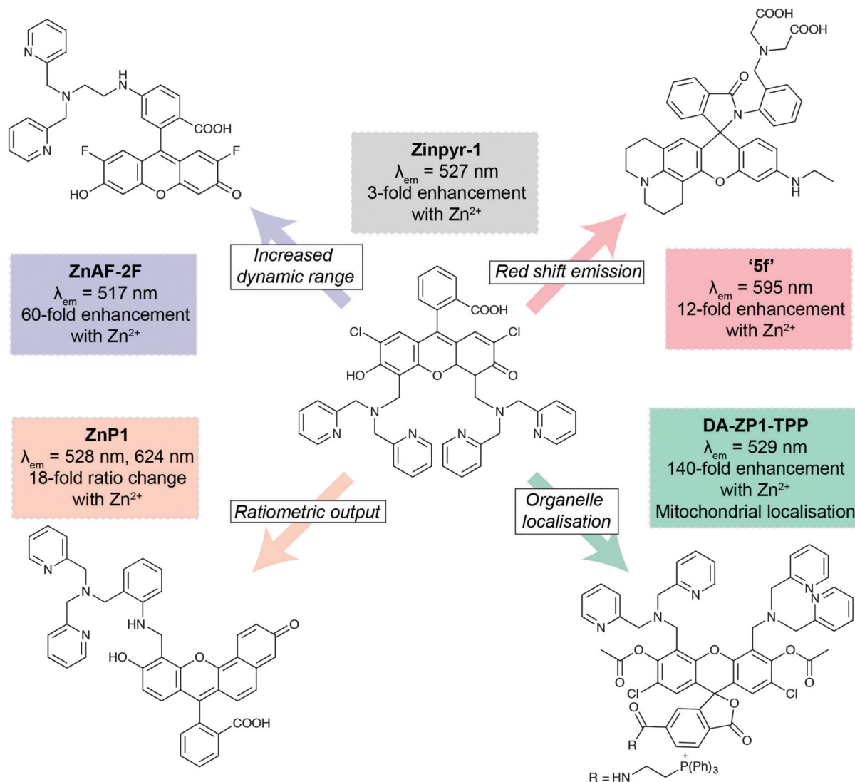
Fig. 6 Key developments in xantheno-based fluorescent sensors for \text{Zn}^{2+} . Zinpyr-1 98 has been further developed to improve the range of \text{Zn}^{2+} concentrations it can detect ( ZnAF-2F ), 99 measure \text{Zn}^{2+} flux via ratiometric measurements ( ZnP1 ), 100 localise within specific organelles, such as mitochondria ( DA-ZP1-TPP ), 101 and optimise its fluorescence emission peak ( 5f ). 102
