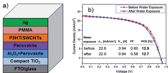
Fig. 6 (a) Schematic illustration of PSC fabricated with CNTs/polymer composite as a hole collection layer as reported by Snaith's group. 79 (b) Current density–voltage curves of PSCs before and after water exposure for 60 s (reprinted with permission from ref. 79 © 2014, American Chemical Society).
