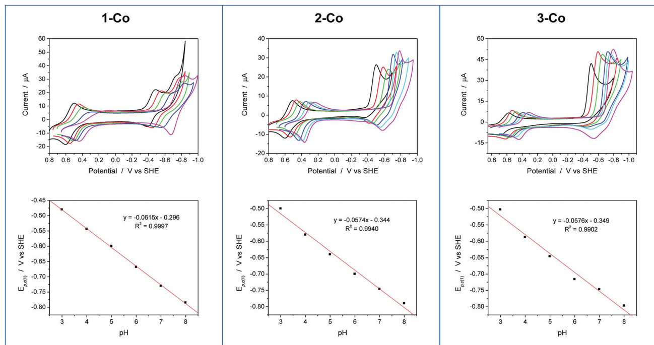
Fig. 5 Cyclic voltammograms as a function of pH and plots of the first reductive peak potential ( E_{p,Co(1)} ) vs. pH for 1-Co, 2-Co, and 3-Co. Conditions: 0.9 mM catalyst, 0.03 M buffer, 0.1 M KNO_3 , 100 mV s^{-1} scan rate, glassy carbon electrode (3 mm dia). Note: CV at pH 7 is omitted for clarity in series of CVs for 1-Co. Legend: pH 3 (black), pH 4 (red), pH 5 (green), pH 6 (blue), pH 7 (cyan), pH 8 (magenta).
