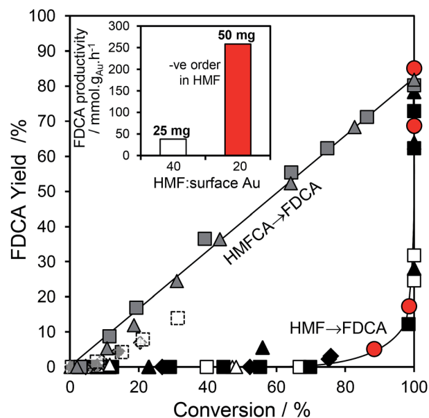
Fig. 5 (main) Disparate evolution of FDCA yield as a function of either HMF or HMFCa conversion over 25 mg \Delta (0.5 wt%), \blacklozenge (1 wt%), \square (2 wt%), \blacksquare (5 wt%), and \blacktriangle (10 wt%) Au/HT catalysts, and 50 mg \bullet (2 wt%) Au/HT; (inset) normalised FDCA productivity per Au atom as a function of HMF : surface Au molar ratio for 2 wt% Au/HT highlighting self-poisoning by high HMF concentrations.
