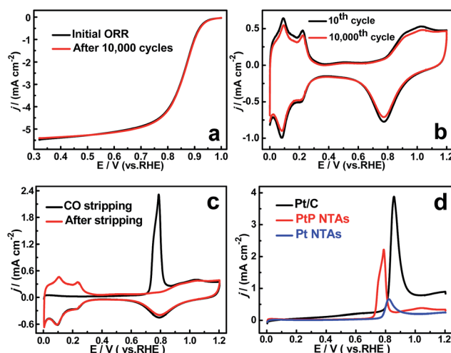
Fig. 4 (a) ORR polarization curves before and after 10 000 potential cycles between 0.6 V and 1.0 V for the PtP NTAs in O_2 -saturated 0.1 M HClO_4 . (b) Cyclic voltammograms curves for the 10th and 10 000th cycles of the PtP NTAs ( 40 \mu\text{g cm}^{-2} ) in N_2 -purged 0.5 M H_2SO_4 . (c) CO stripping voltammograms of the PtP NTAs performed in 0.5 M H_2SO_4 solution at 50 \text{ mV s}^{-1} . (d) The comparison of CO stripping voltammograms of the PtP NTAs, Pt NTAs, and Pt/C (JM) (Pt loading: \sim 28 \mu\text{g cm}^{-2} ).
