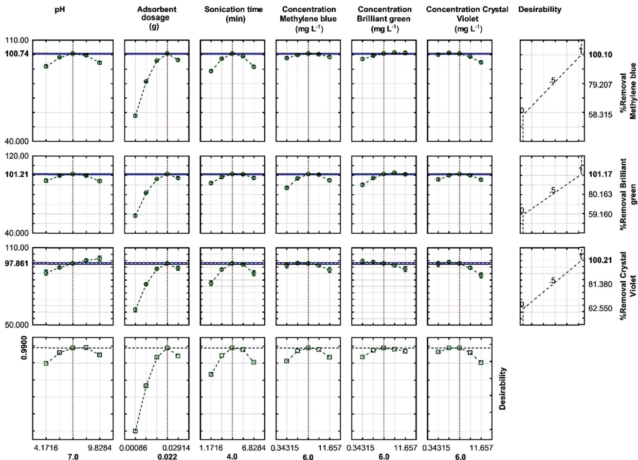
Fig. 9 Profiles for the predicted values and desirability function for the removal percentage of MB, BG and CV. The dashed lines indicate the current values after the optimization process.
