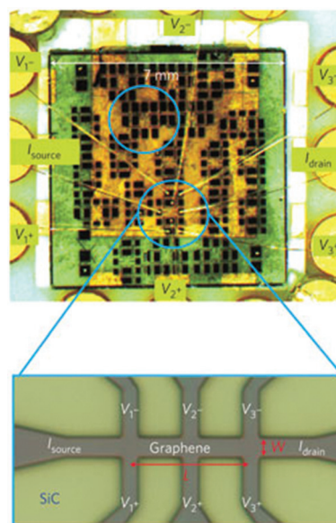
Fig. 33 7 \times 7 mm 2 wafer of SiC with 20 Hall bar devices. The contact configuration for the smaller device is shown in the enlarged image. 154
