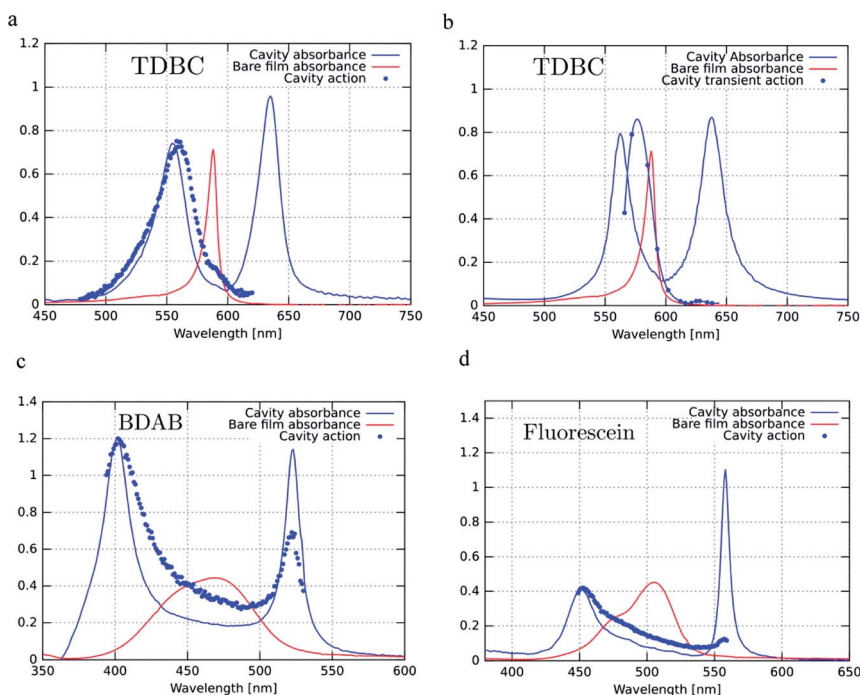
Fig. 4 Excitation or action spectra (blue dots) recorded at normal incidence for P − emission for (a) TDBC (at 680 nm), (c) BDAB (at 540 nm) and (d) Fluorescein (at 576 nm) and (b) for P − transient absorption of TDBC. These spectra are compared to the bare molecule absorbance spectra (solid red lines) and the strongly coupled system absorbance spectra (solid blue lines) of the same samples.
