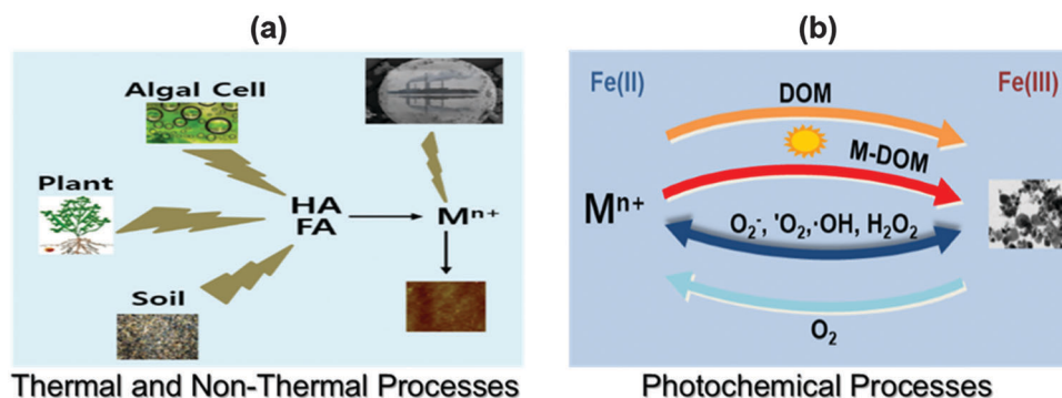
Fig. 2 (a) Thermal and non-thermal processes and (b) photochemical processes that generate natural nanoparticles in the environment (for details see Section 2). (HA – humic acid; FA – fulvic acid; DOM – dissolved organic matter; \text{M}^{n+} – metal ions (e.g., \text{Ag(I)} and \text{Au(III)} ); M-DOM – metal ion complexation with dissolved organic matter).
