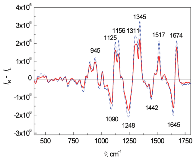
Fig. 3 Average Raman spectra of human blood plasma samples: control group (dotted line) and colon cancer patients (solid line).
