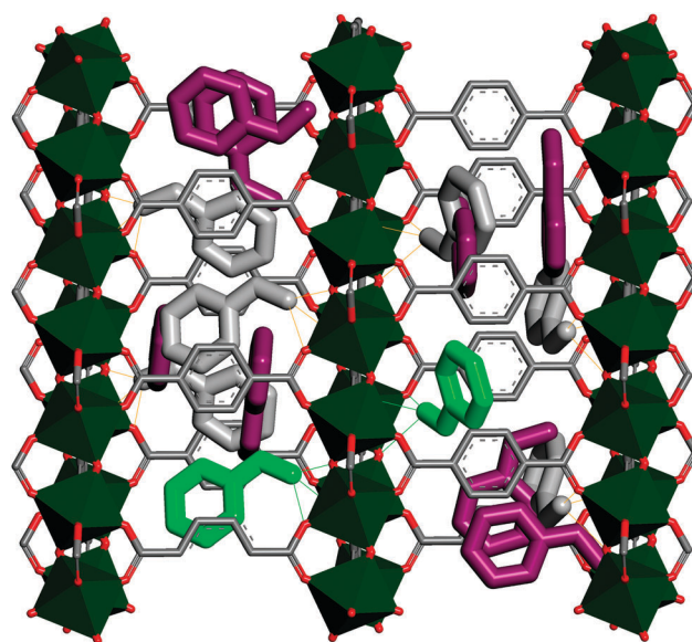
Fig. 17 Stacking of ethylbenzene in styrene-loaded MIL-47. Styrene (purple) is packed pairwise in the channels of MIL-47, occupying several adsorption sites of ethylbenzene (gray). Only two of the possible adsorption sites for ethylbenzene are occupied (green). 94
