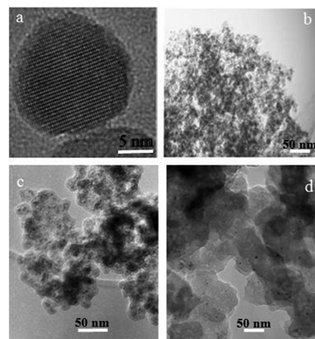
Fig. 3 TEM images of (a, b) \gamma -Fe 2 O 3 MNPs 1 , (c) iodoalkyl-functionalized SiO 2 -coated MNPs 3 and (d) neocuproine functionalized SiO 2 -coated MNPs 7 .
