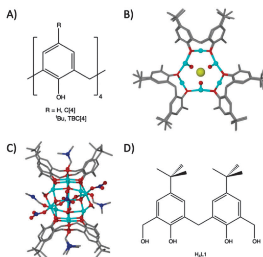
Fig. 1 (A) General calix[4]arene framework. (B) Tri-capped trigonal prismatic [Cu II 9 (TBC[4]) 3 ]Cl 2 cluster, viewed down the face of the prism. 4 (C) Cu 11 cluster formed with tetrahomodioxacalix[4]arene. 12 (D) Schematic of H 4 L 1 .
