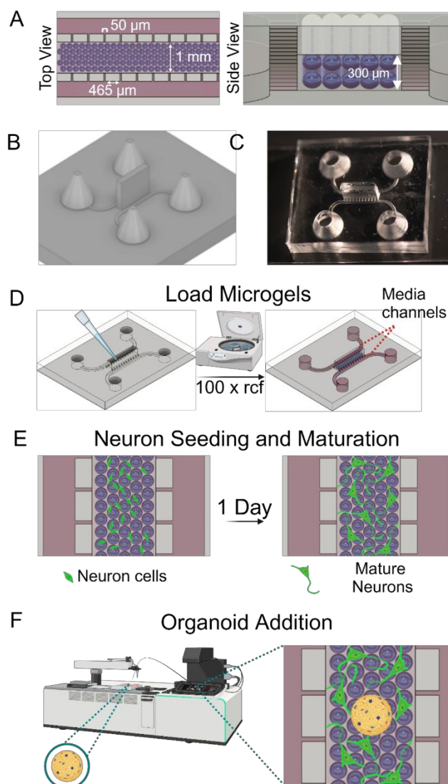
Figure 1. Device design and schematics. (A) Schematic of top and side views of the device loaded with microgels. (B) CAD drawing of the negative master-mold. (C) Photograph of the device. (D-F) Schematic of how microgels are loaded into the device, neurons are cultured, and organoids are added to the device.
