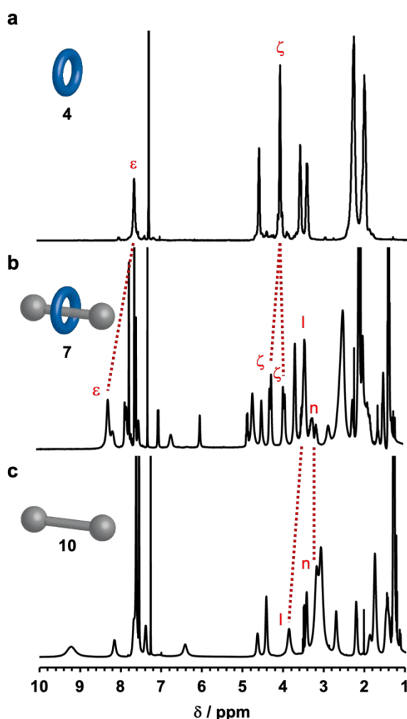
Fig 2. 1 H NMR spectra (400 MHz, CDCl 3 , 298.15 K) of (a) cyclo(PG) 4 , (b) [2]rotaxane 7 , and (c) monocationic ammonium thread 10 . The peaks are labeled according to Scheme 1. The complete attribution of each NMR spectrum is detailed in the Supporting Information (Fig S15-S17).
