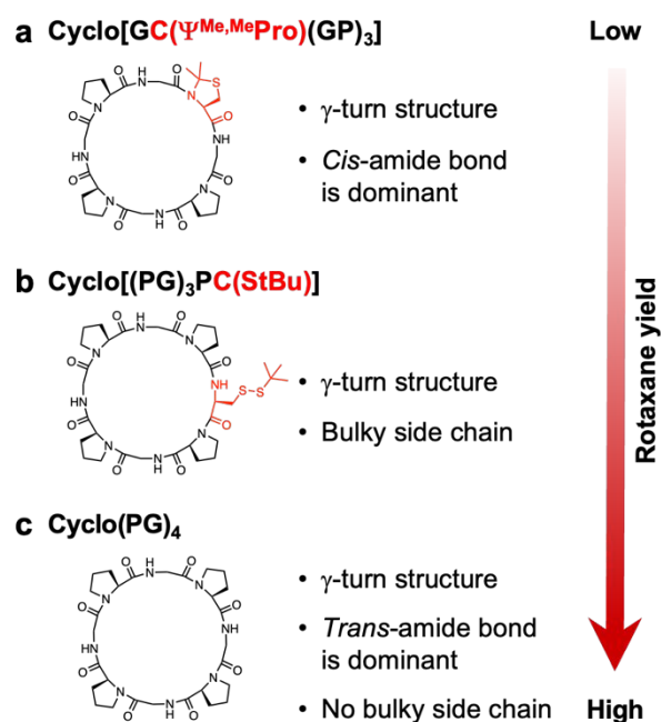
Fig 5. Summary diagram of the effects of the cyclic peptide amino acid sequence on rotaxane formation in this study. (a) Cyclo[GC(Ψ Me ,MePro)(GP) 3 ], which adopts a γ-turn structure with predominantly cis -amide bonds (Table 2), was unable to form a rotaxane. (b) Cyclo[(PG) 3 PC(StBu)], which adopts γ-turn structure with bulky side chains, formed a rotaxane in a low yield. (c) Cyclo(PG) 4 , which adopts a γ-turn structure with predominantly trans -amide bonds (Table 2) and lacks bulky side chains, demonstrated the highest produced a rotaxane in the highest yield to date. This figure underscores how strategically modifying the amino acid sequence modifications in of a cyclic peptide can significantly enhance rotaxane yield. Moreover, continued optimization of these cyclic peptides has the potential to achieve even greater improvements in could lead to further improvements in rotaxane yield.
