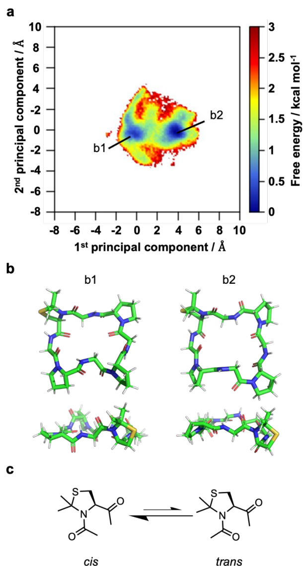
Fig 4. (a) Free energy landscape of cyclo[GC( \Psi^{\text{Me,Me}}\text{Pro} )(GP) 3 ] determined by PCA. (b) Molecular structures of the two main representative metastable states of cyclo[GC( \Psi^{\text{Me,Me}}\text{Pro} )(GP) 3 ]. (c) Schematic of proline cis-trans isomerization.
