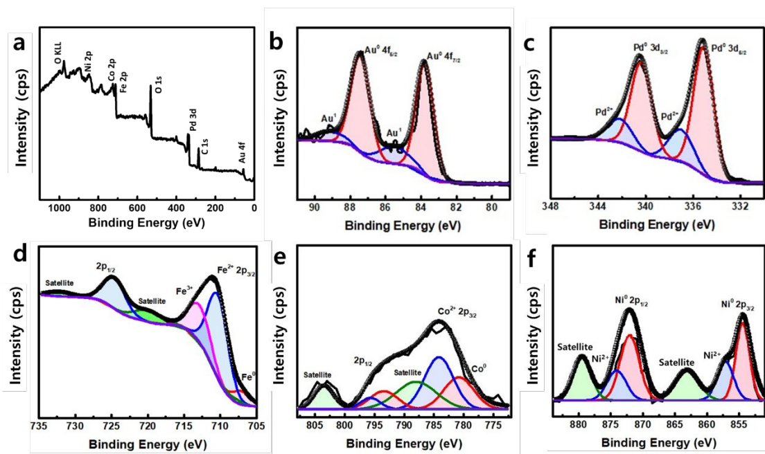
Fig. 3 X-ray photoelectron spectroscopy (XPS) characterization (a) XPS survey spectrum of the synthesized AuPdFeNiCo HEA NPs. High-resolution XPS spectra of (b) Au 4f, (c) Pd 3d, (d) Fe 2p, (e) Co 2p, and (f) Ni 2p.
