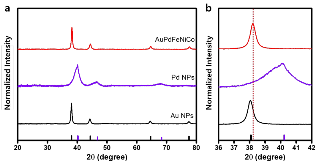
Fig. 2 X-ray diffraction (XRD) characterization of AuPdFeNiCo HEA NPs (a) XRD patterns of Au NPs, Pd NPs and AuPdFeNiCo HEA NPs with JCPDS data (Au: 04-0748, Pd: 46-1043), (b) XRD patterns of (111) fcc peak.
