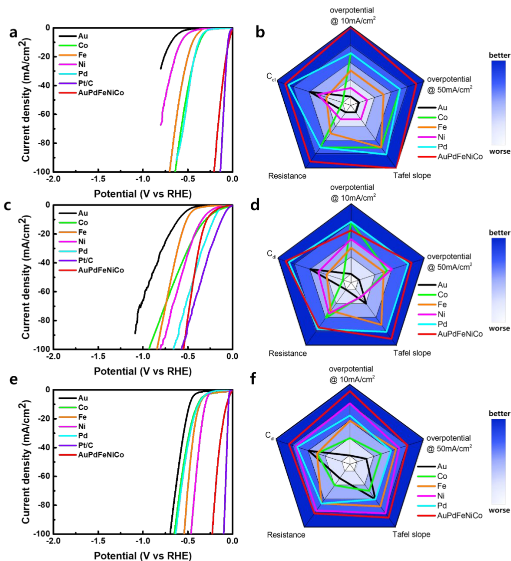
Fig. 4 HER electrocatalysis in acidic, neutral, and alkaline electrolyte. HER polarization curves of Au, Pd, Fe, Ni, Co, AuPdFeNiCo, and Pt/C in (a) 0.5M \text{H}_2\text{SO}_4 , (c) 1M PBS, (e) 1M KOH, corresponding radar chart comparison of the potential characteristics of the electrocatalysts in (b) 0.5M \text{H}_2\text{SO}_4 , (d) 1M PBS, and (f) 1M KOH.
