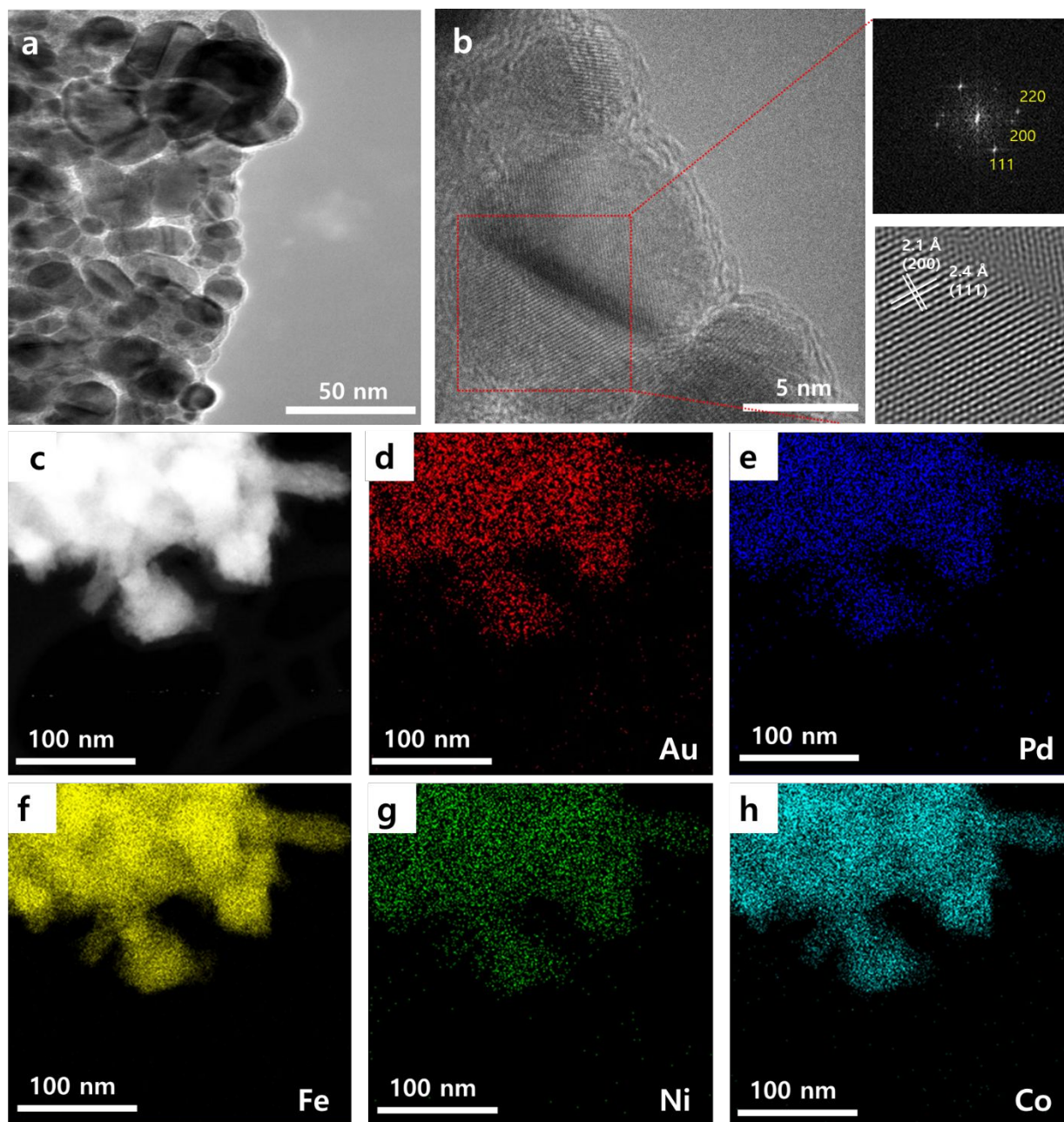
Fig. 1 HR-TEM and STEM-EDS characterization of AuPdFeNiCo HEA NPs (a) Representative HR-TEM image of AuPdFeNiCo HEA NPs and (b) zoomed in view of the HR-TEM image with the insert shows the fast Fourier transformation (FFT). (c) STEM image of the corresponding energy dispersive spectroscopy (EDS) elemental mapping of (d) Au, (e) Pd, (f) Fe, (g) Ni, and (h) Co.
