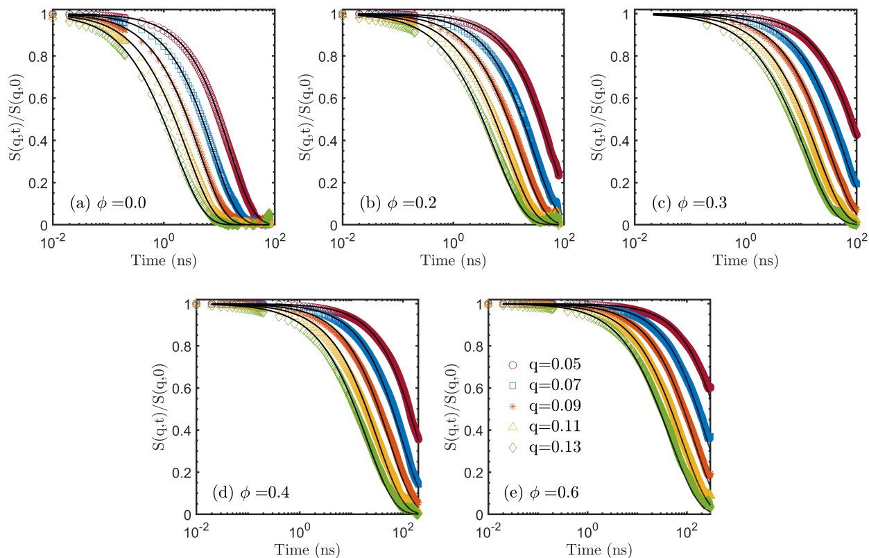
Fig. 8 Dynamic structure factor. q is from 0.05 to 0.13 with a step size of 0.02 in calculating the dynamic structure factor. The symbols are the results of using Eq. 7 on trajectories from MD simulations. The solid curves are estimations according to Eq. 8. There is no fitting involved.
