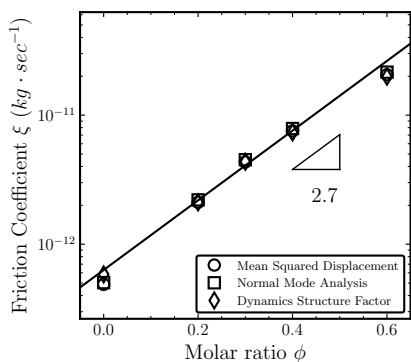
Fig. 9 Monomeric friction coefficients. The coefficients are estimated from all three analyses. The scaling factor of 2.7 is indicated.
